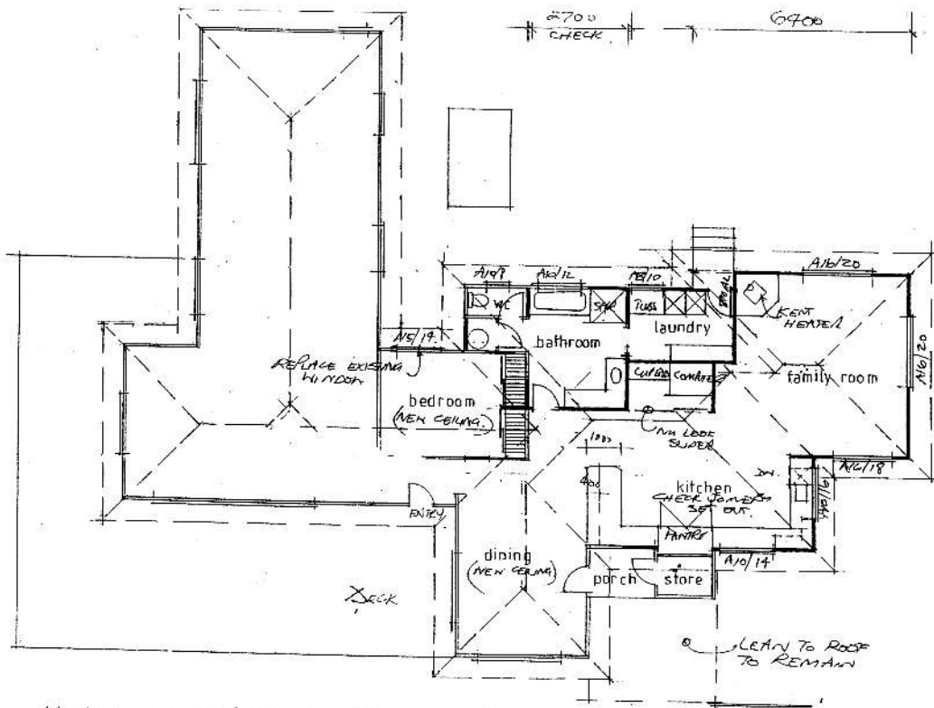
1st RE-ARRANGING of ORIGINAL FARMHOUSE - scale 1/100
